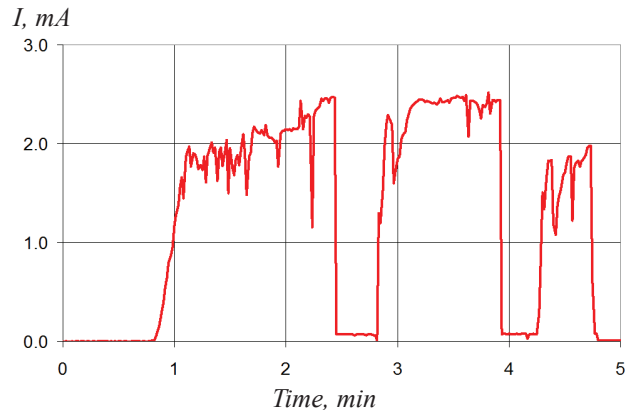
Figure 4: Output ion current in the experiments on high current transportation.
