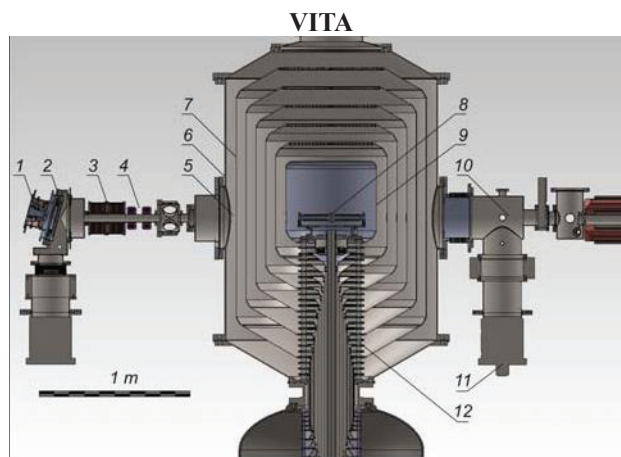
Figure 1: High-current vacuum insulation tandem accelerator. 1 – \text{H}^- ion source, 2 – diaphragm, 3 – magnetic lenses, 4 – corrector, 5 – aperture of the first electrode, 6 – accelerator body, 7 – electrodes, 8 – stripper, 9 – high voltage electrode, 10 – high energy beam transporting channel, 11 – turbo molecular pumps, 12 – insulator.
