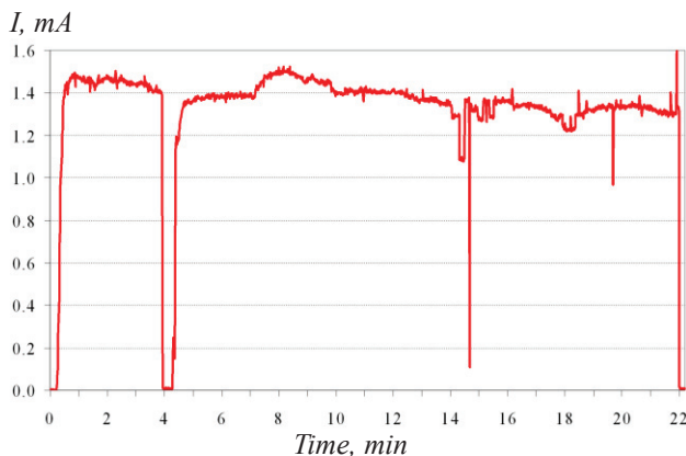
Figure 3: Output proton current in the experiments on high current transportation.
