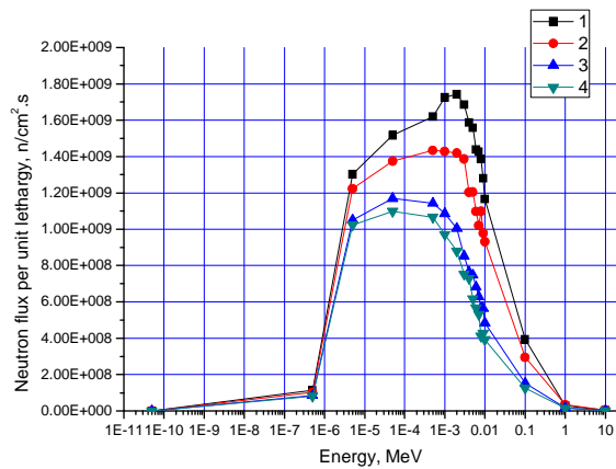
Fig.1. Neutron spectra at the beam exit for the base model (1) and F/M built of 0,81 m ^{27}\text{Al} and 0,13 m \text{Al}_2\text{O}_3 (2); 0,83 m ^{27}\text{Al} and \text{Al}_2\text{O}_3 (3); 0,83 m ^{27}\text{Al} and 0,17 m \text{Al}_2\text{O}_3 (4)
