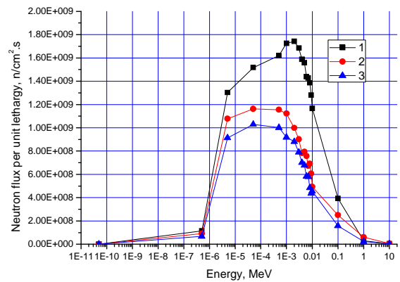
Fig. 2. Neutron spectra at the beam exit for the base model (1) and F/M built of 0,81 m ^{27}\text{Al} and 0,16 m ^{12}\text{C} (2); 0,96 m ^{27}\text{Al} and 0,12 m ^{12}\text{C} (3)
