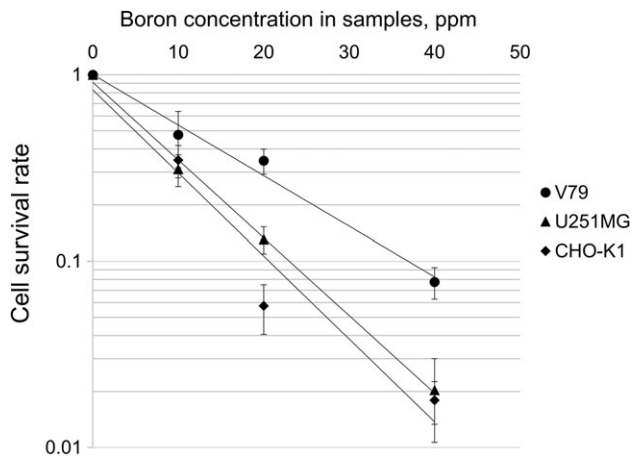
Fig. 4. Cell survival curves depend on the boron concentration in the samples. The data are presented as means \pm SDs. * P < 0.01 with respect to boron concentration of 0 ppm (one-way ANOVA).
