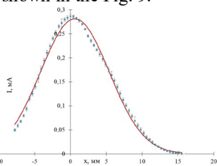
Figure 9: The dependence of the proton beam current, passed through the hole from its coordinate on the collimator and Gaussian distribution, approximated this dependence.
