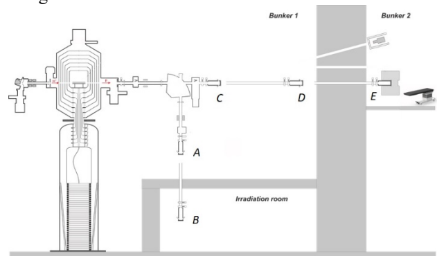
Figure 1: A diagram of an accelerator based source of epithermal neutrons. A-E – sites of the lithium neutron generating target.
