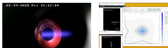
Figure 6: H + beam entering the accelerator (left) and soft, estimating the proton beam size and profile (right).
